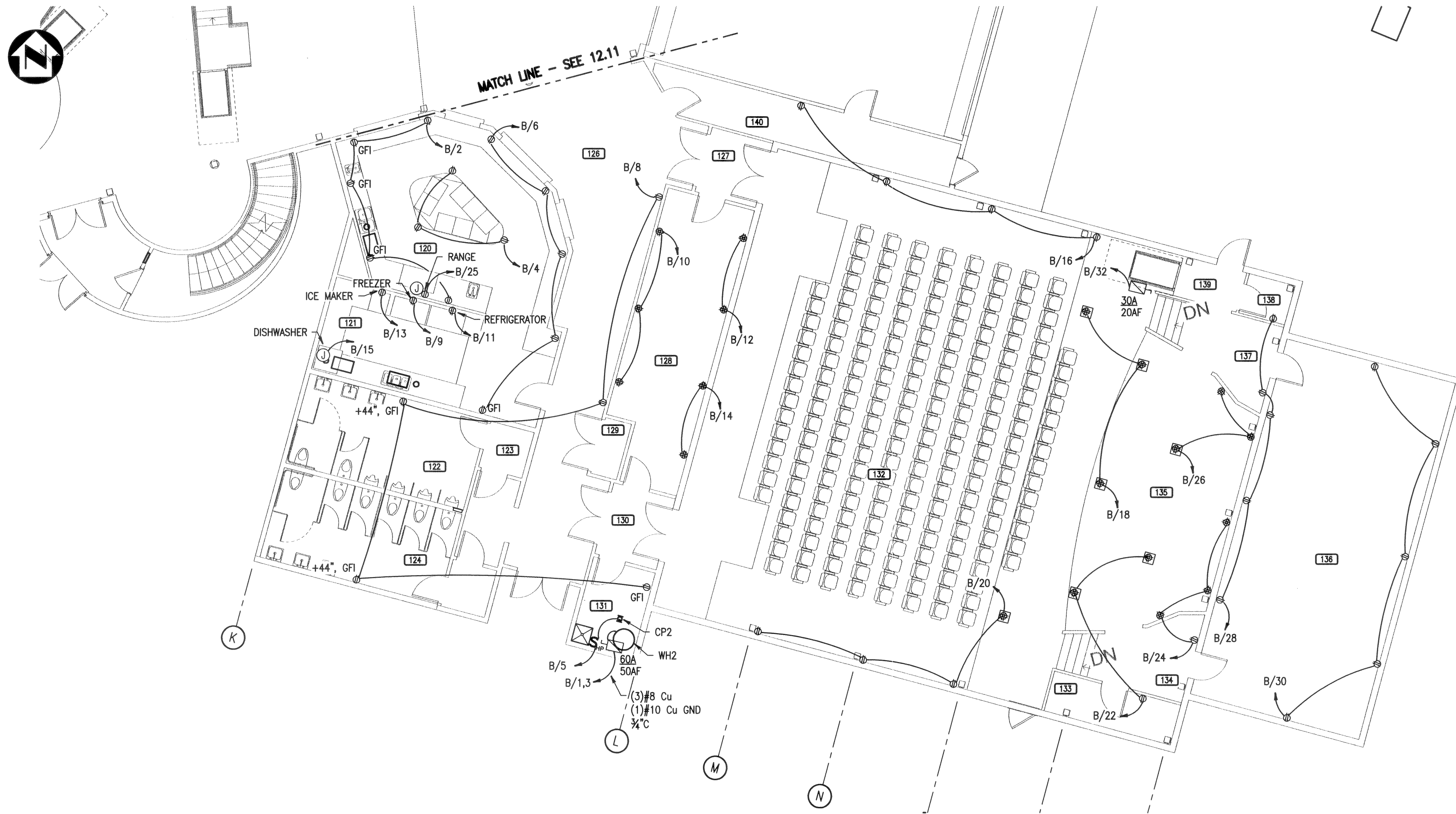
MAIN LEVEL POWER PLAN
