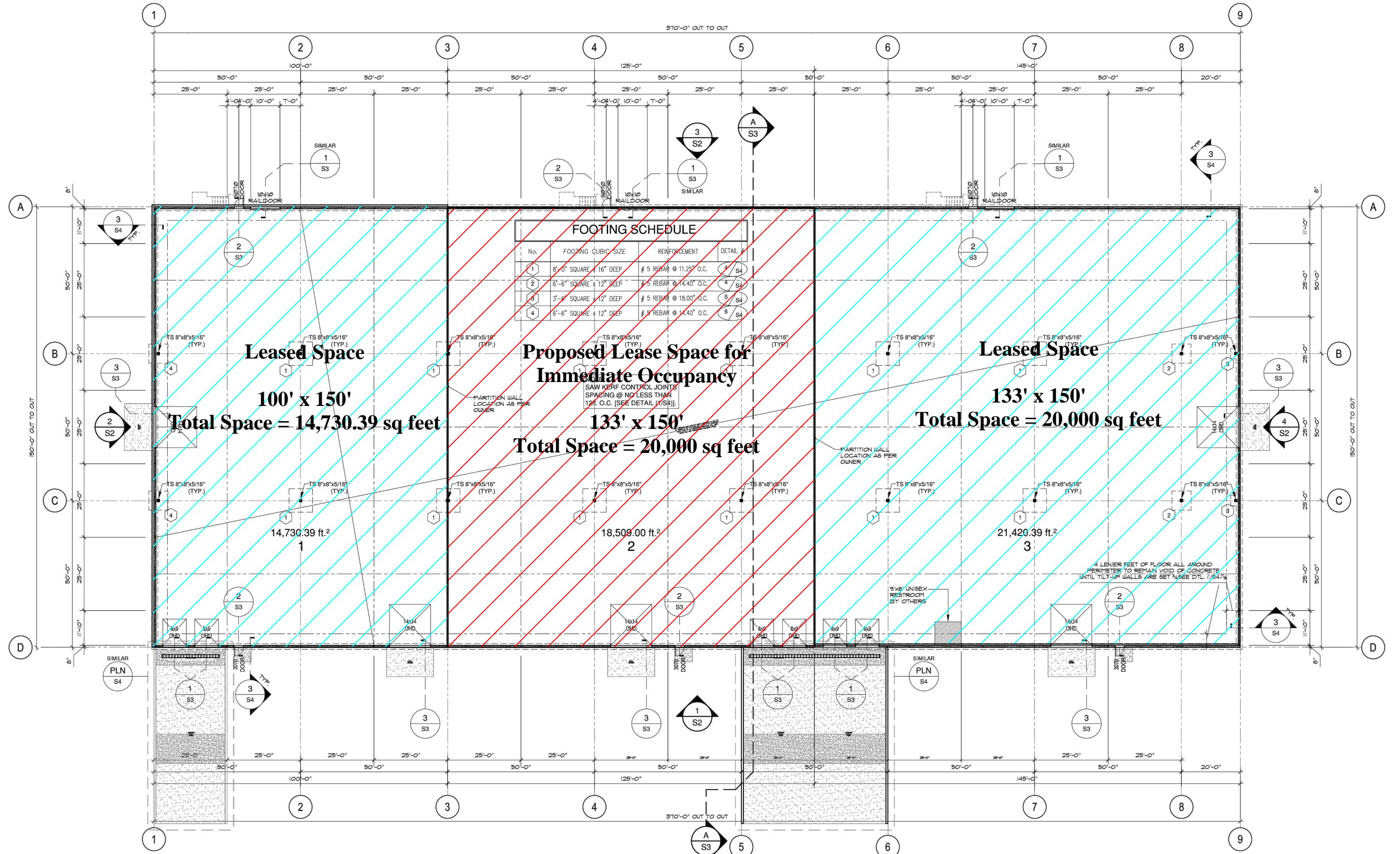
ROOF FRAMING PLAN SCALE: 1/16"=1'-0"
